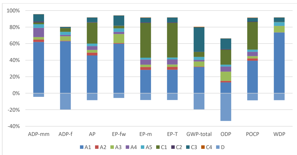
Figure 2: Tensar® TriAx® TX190L - Impact of the individual modules on the environmental core indicators (NMD set 2)
